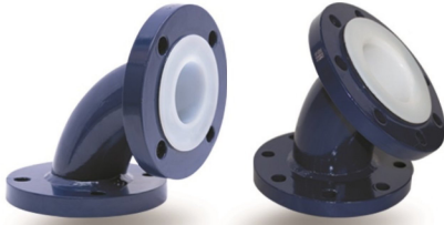
LINED ELBOW (90° & 45°) SIZE: 0.5" TO 20"
